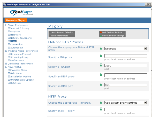
With the included Configuration Tool, you configure a range of items in RealPlayer Enterprise, including proxy settings, minimum and maximum bandwidths, player preferences and more,
